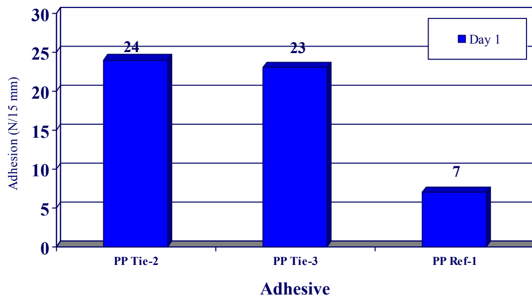
Figure (11): Drop Test Results for PP Based Tie Layers in Bottle Applications
