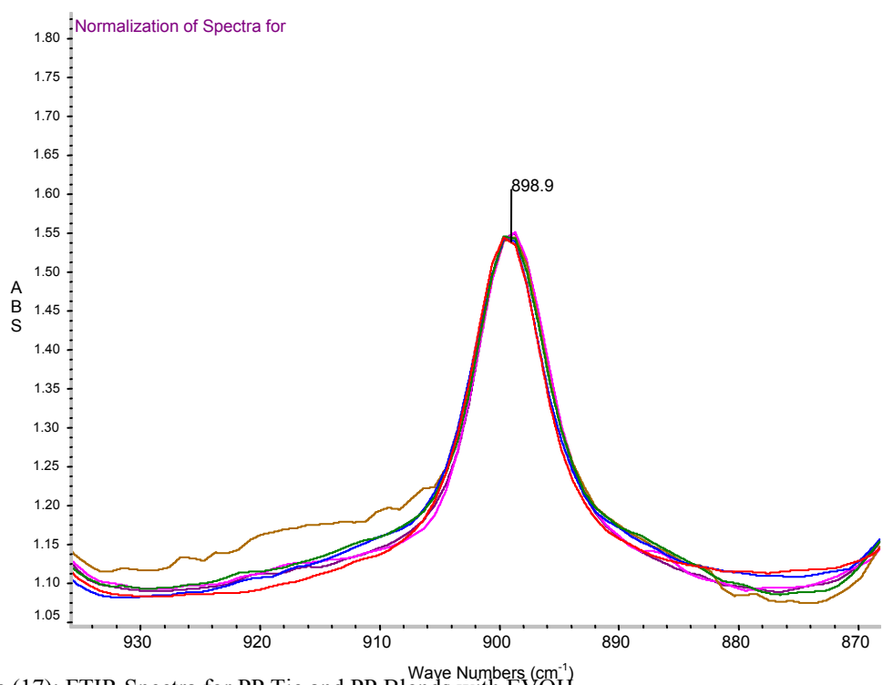
Figure (16): Thickness Normalization of FTIR Spectra for PP Tie and PP Blends with EVOH
