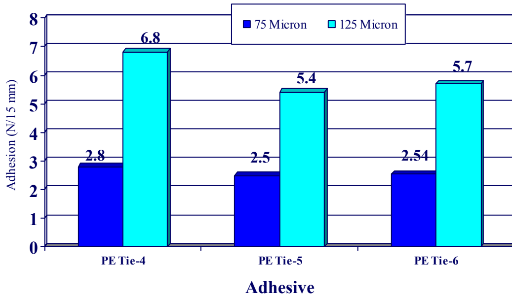
Figure (8): Adhesion at Tie-Layer / EVOH Interface for PE Based Tie Layers of Series - 2
