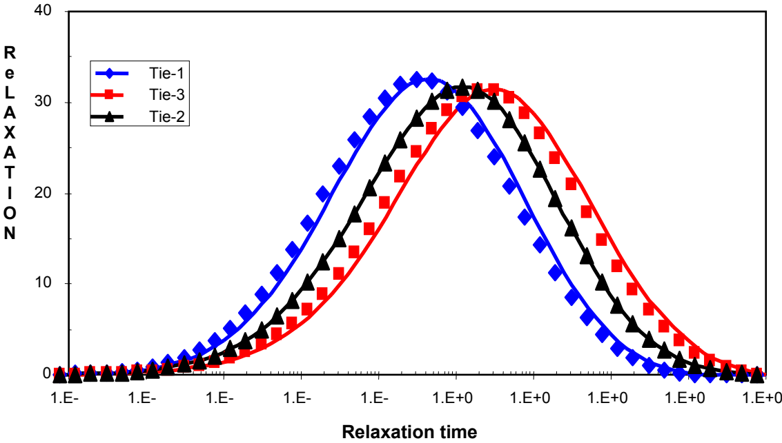
Figure (5): Adhesion at Tie-Layer / EVOH Interface for PE Based Tie Layers of Series - 1
