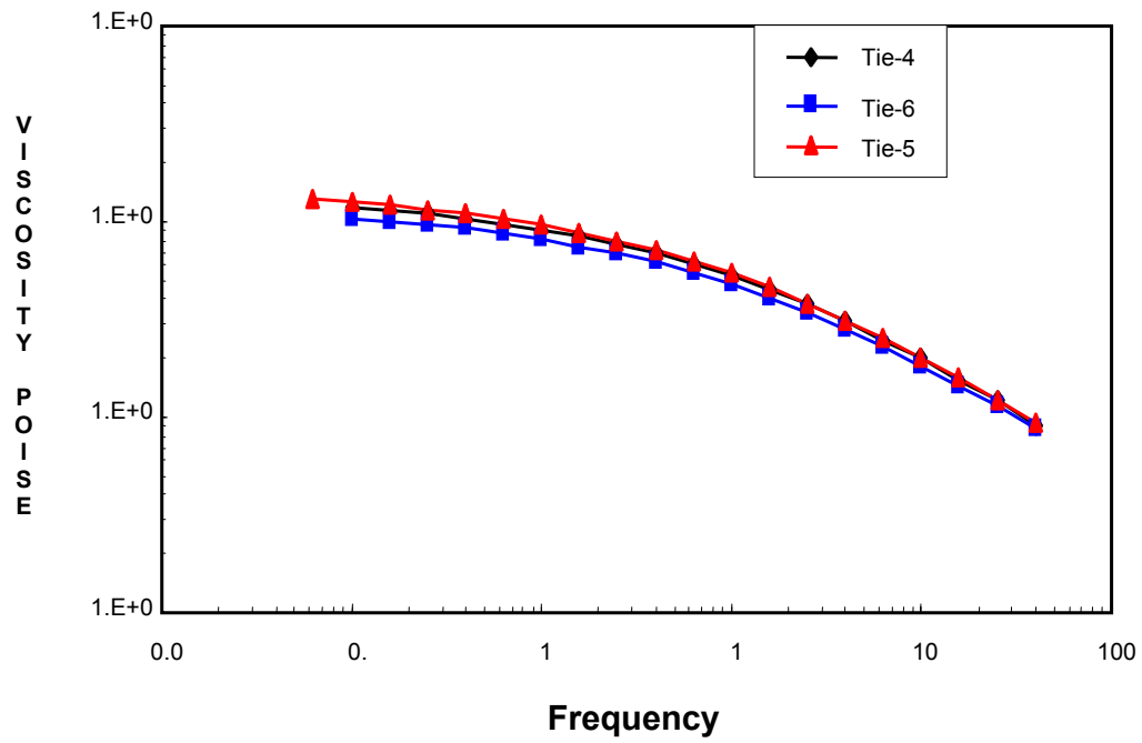
Figure (6) Viscosity Comparison
