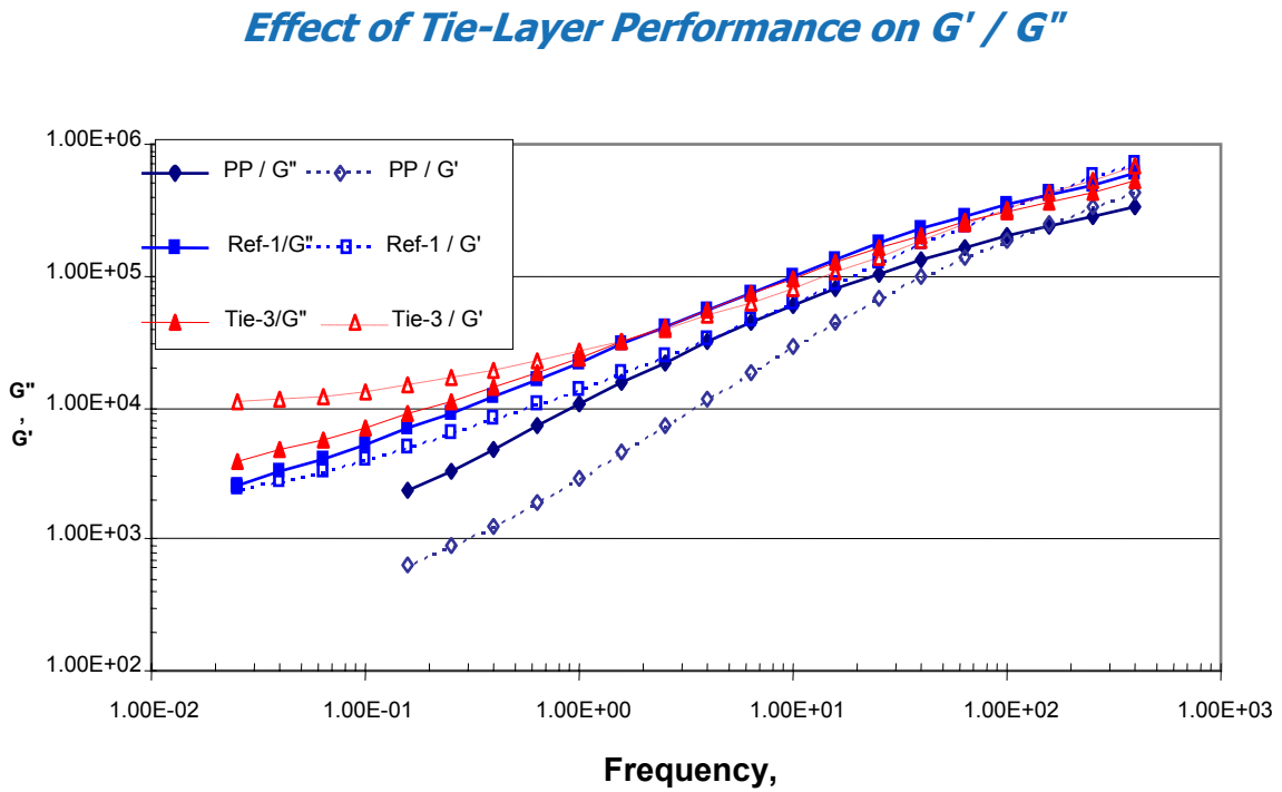
Figure (15): G'/G'' versus Frequency for PP-Based Tie Layer Blends with EVOH
