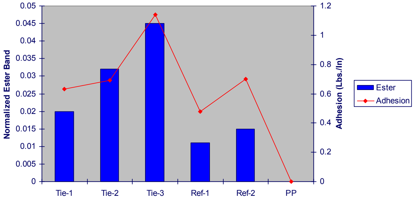
Figure (19): Correlation between Adhesion and Acid Formation in PP Tie / EVOH Structures
