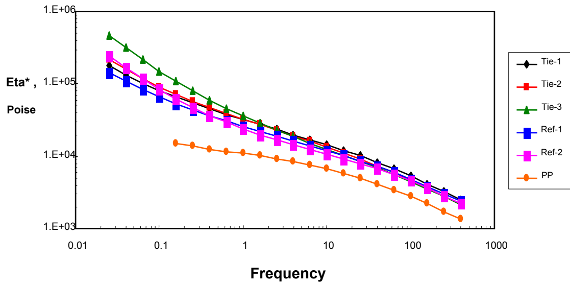
Figure (13): G' versus Frequency for PP-Based Tie Layer Blends with EVOH
