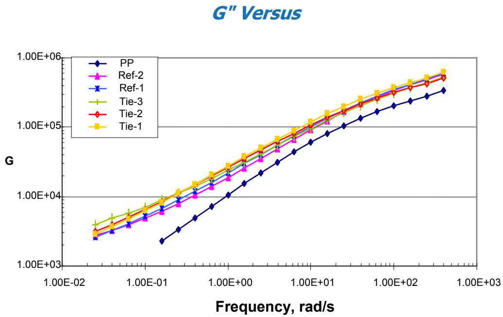
Figure (15): G'/G'' versus Frequency for PP-Based Tie Layer Blends with EVOH
