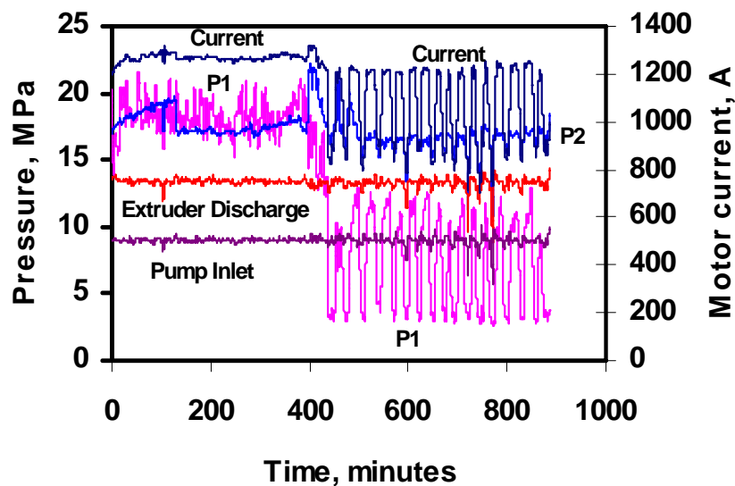
Figure 3. Barrel, discharge, and pump inlet pressures and motor current for stable and unstable extrusion for a large-diameter extruder running HIPS resin.
