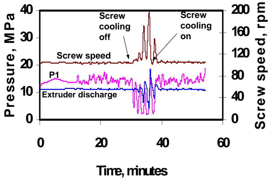
Figure 7. Screw speed, pressure at the entry to the first-stage meter (P1), and discharge pressure for the screw cooling experiment.
