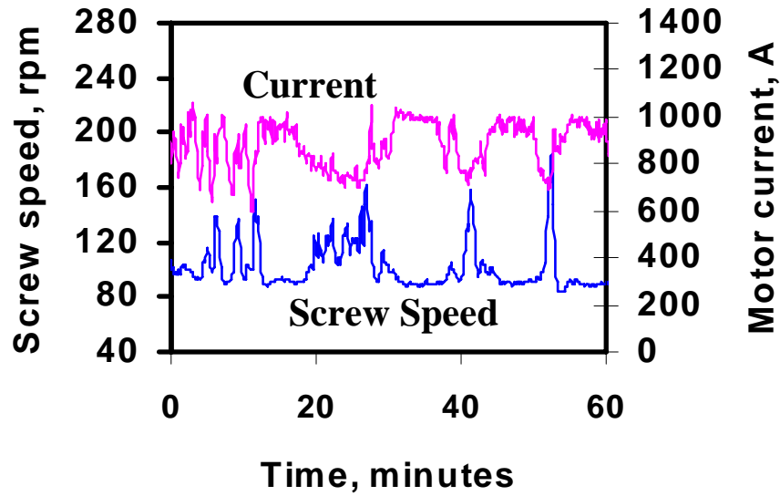
Figure 7. Screw speed and motor current for a large-diameter extruder with a feed casing that was too hot.
