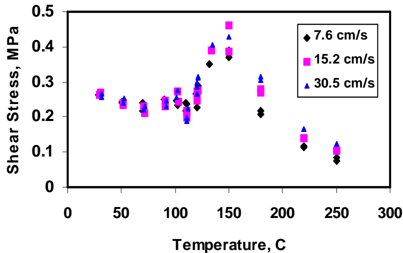
Figure 1. Shear stress between HIPS resin and a metal surface at 0.7 MPa and as a function of sliding velocity.
