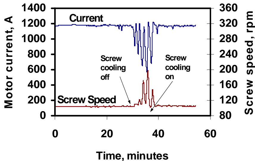
Figure 6. Screw speed and motor current for the screw cooling experiment.
