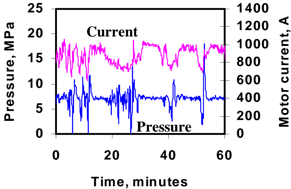
Figure 8. Discharge pressure and motor current for a large-diameter extruder with a feed casing that was too hot.
