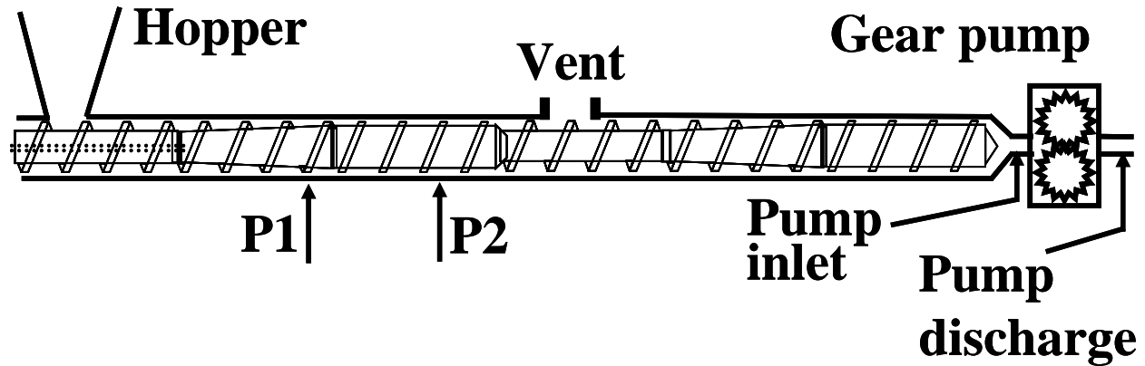
Figure 2. Schematic of the extrusion process.
