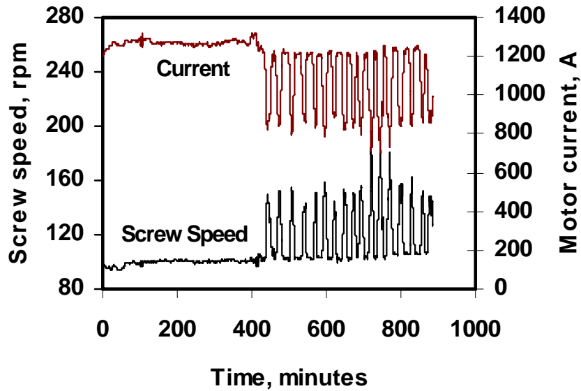
Figure 4. Screw speed and motor current for a large-diameter extruder running stable and unstable.
