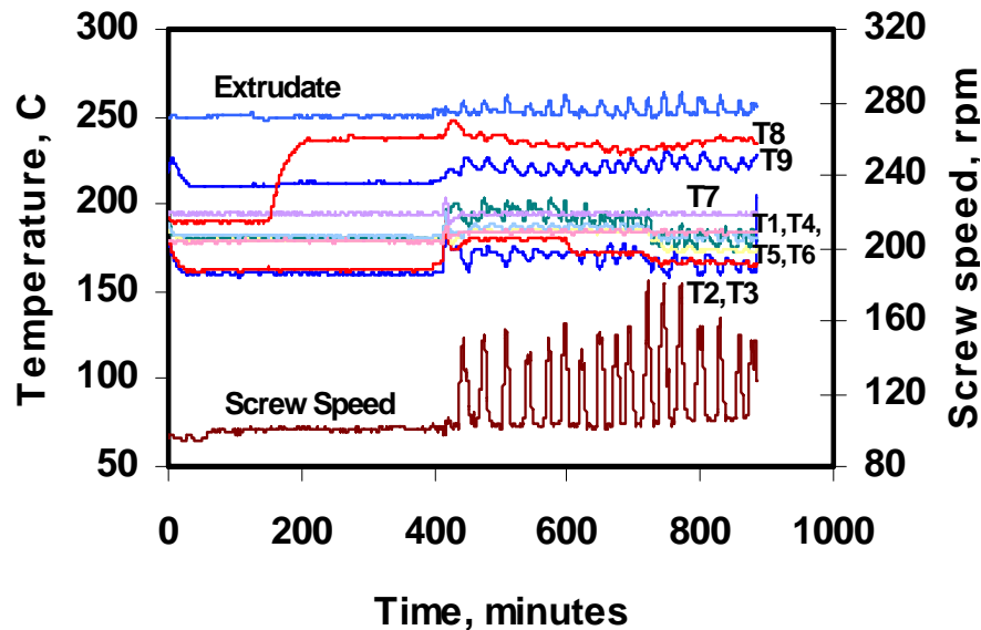
Figure 5. Screw speed, extrudate temperature, and barrel zone temperatures for a large-diameter extruder running stable and unstable.
