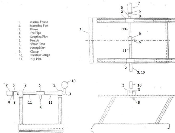
Fig. 1. Spray washer.
