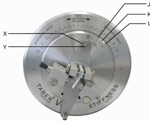
Fig. 2. Stiffness instrument
