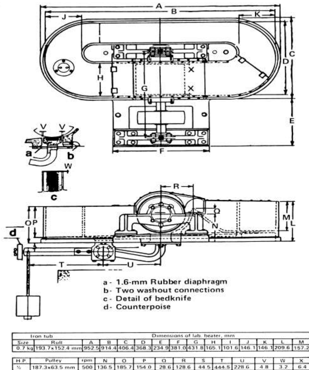
Fig. 1. Beater with controlled bedplate.
